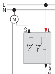
Rollladentaster, 1-polig MEG3755-0000
